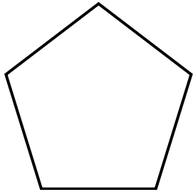
pentagon
