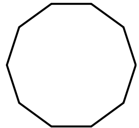
decagon
