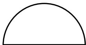
semicircle
