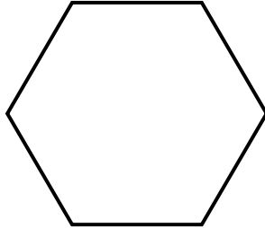
hexagon
