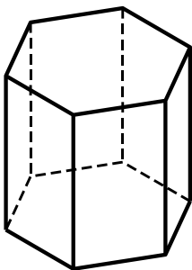
hexagonal prism
