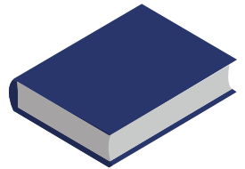
cuboid
