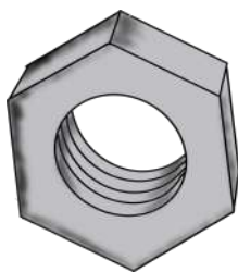
hexagonal prism
