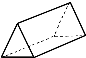
triangular prism
